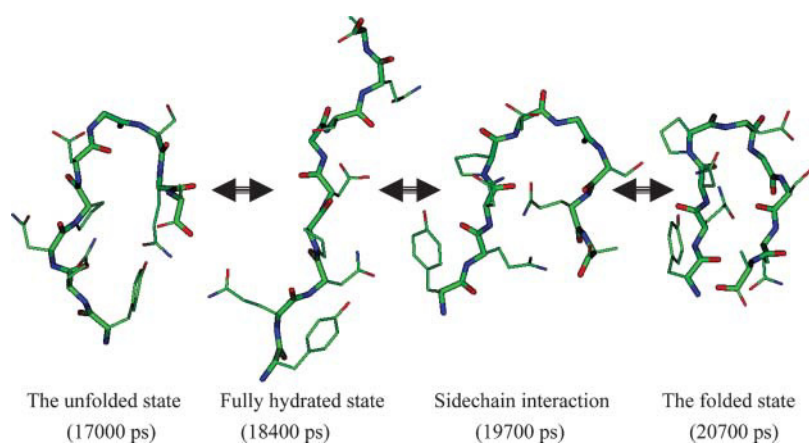
FIGURE 10 Typical conformational changes during a \beta -hairpin folding. The conformation at 17,000 ps represents an unfolded structure with some intrapeptide interactions. At 18,400 ps the peptide becomes fully hydrated. Side-chain interactions bring the two strands together at 19,700 ps. At 20,700 ps the peptide reaches a \beta -hairpin structure. Only heavy atoms are shown. Backbone atoms are shown as thick sticks. Atoms are colored as described in the legend of Fig. 2.
