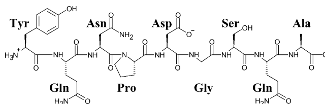
Tyr1-Gln2-Asn3-Pro4-Asp5-Gly6-Ser7-Gln8-Ala9
